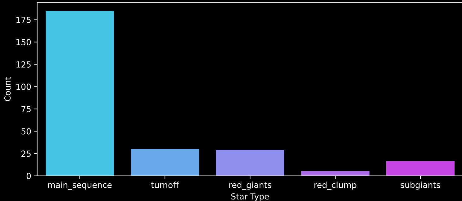
APOGEE DR17 Field: [sgr_tidal5] Count plot of Star Type
