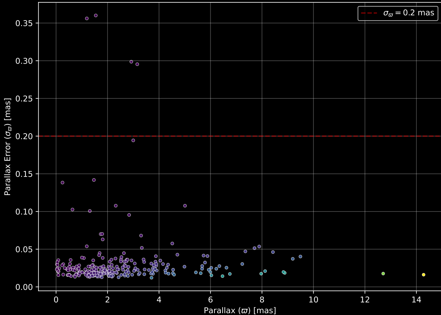
APOGEE DR17 Field: [sgr_tidal5] Parallax Quality (n= 265)
