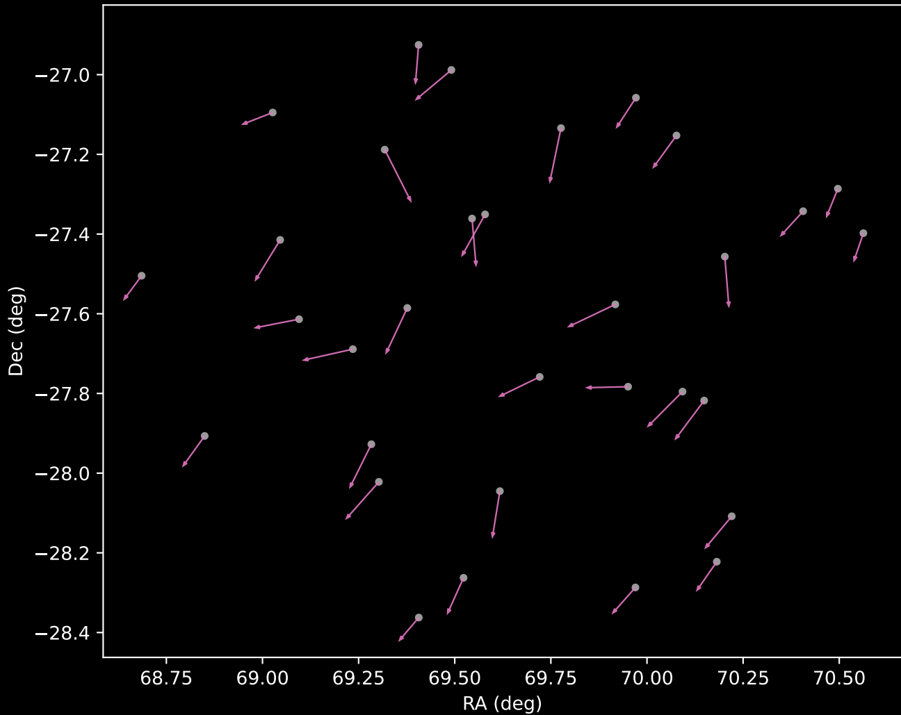
APOGEE DR17 Cluster 12 Proper Motion Vectors (n=32)
