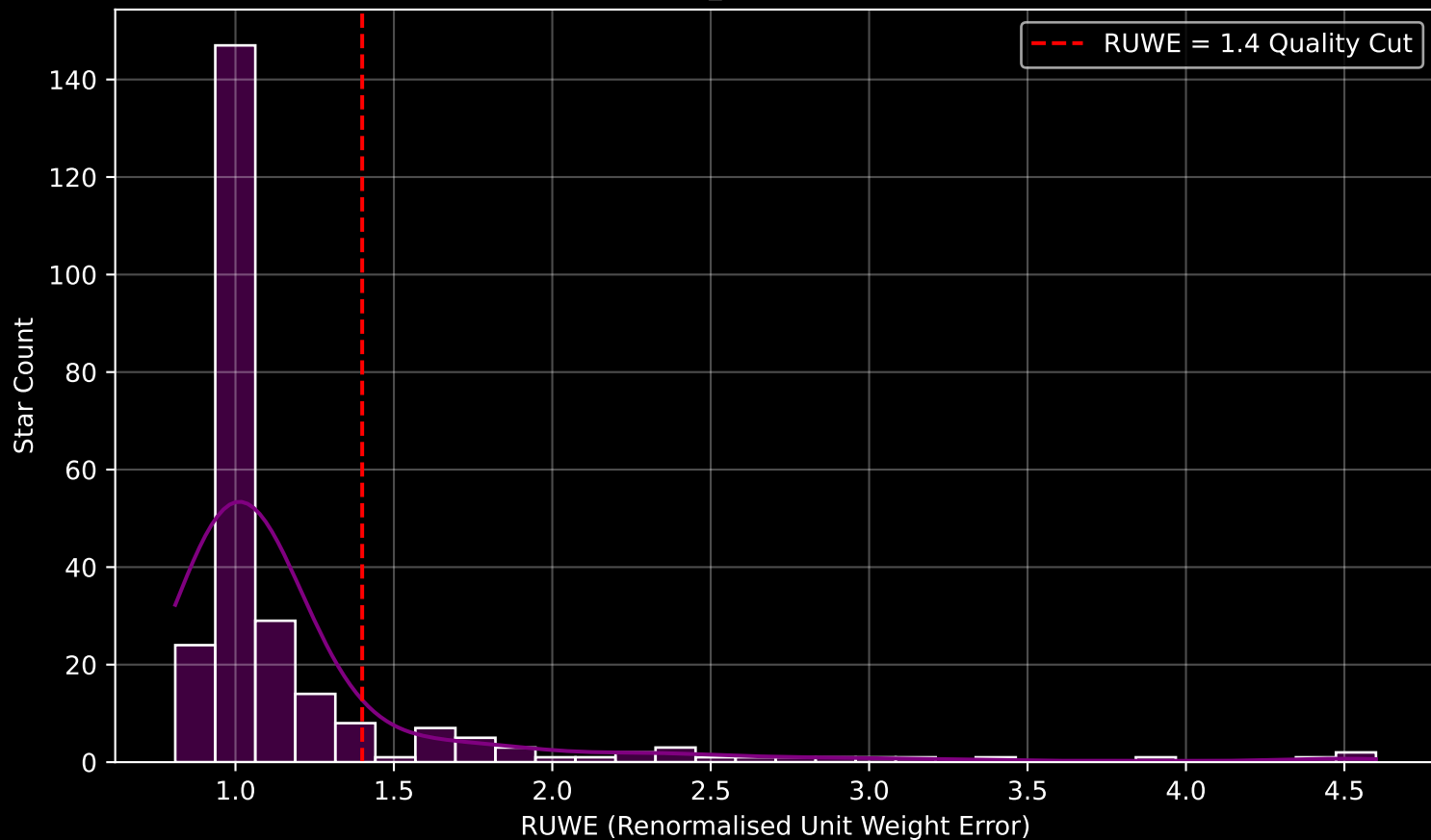
GAPOGEE DR17 Field [sgr_tidal5] RUWE Distribution (n= 256)
