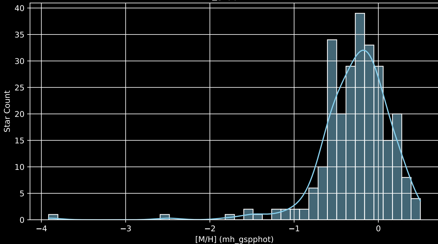
APOGEE DR17 Field: [sgr_tidal5 [M/H] (mh_gspphot) (n= 261)
