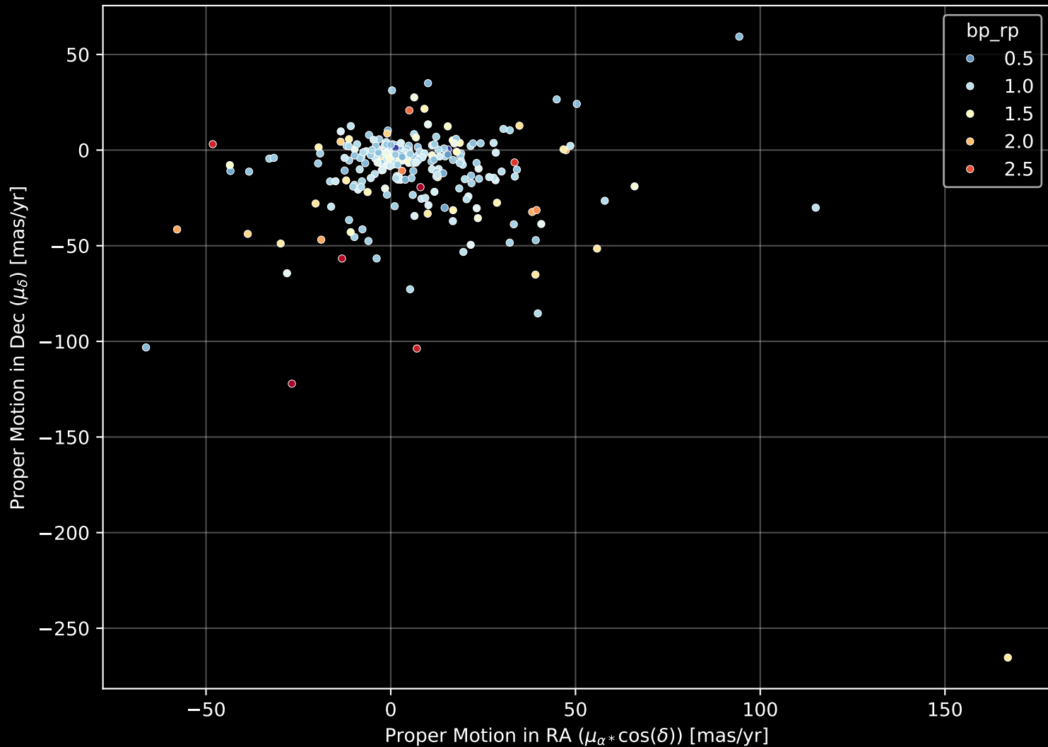
APOGEE DR17 Field: [sgr_tidal5] Proper Motion Diagram (n= 265)
